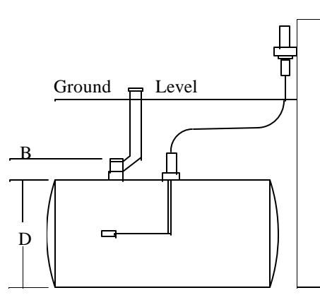
Fig.-2 DU - Underground Installation
